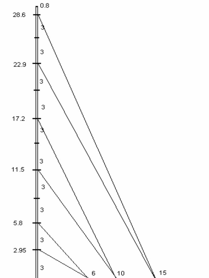
2. Figure: 30m Tower assembly and guy wire levels.
