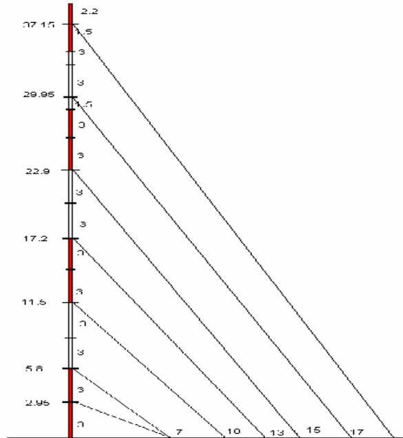
2. Figure: 45m Tower assembly and guy wire levels.
